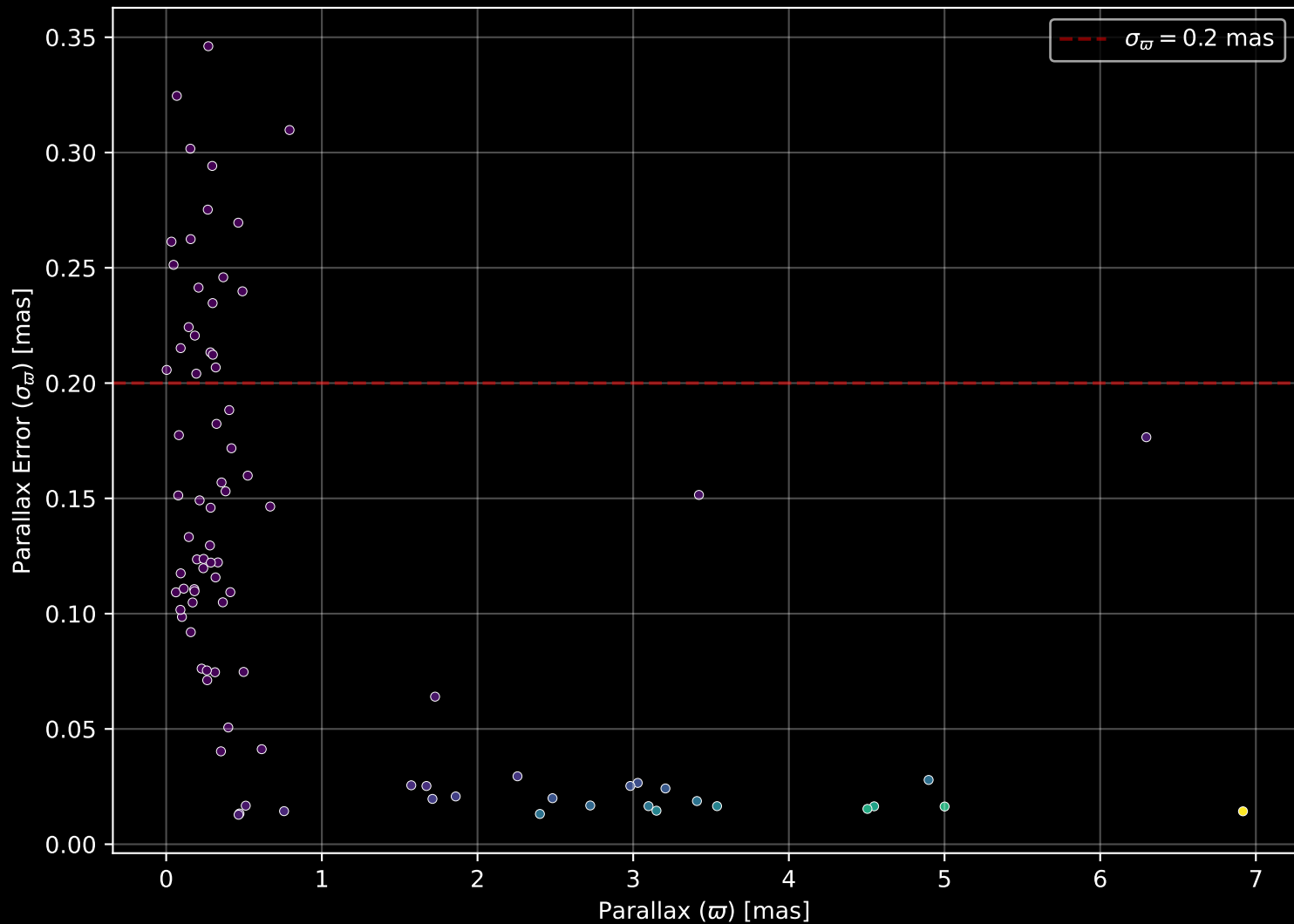
APOGEE DR17 Field: [030+00_btx] Parallax Quality (n= 87)
