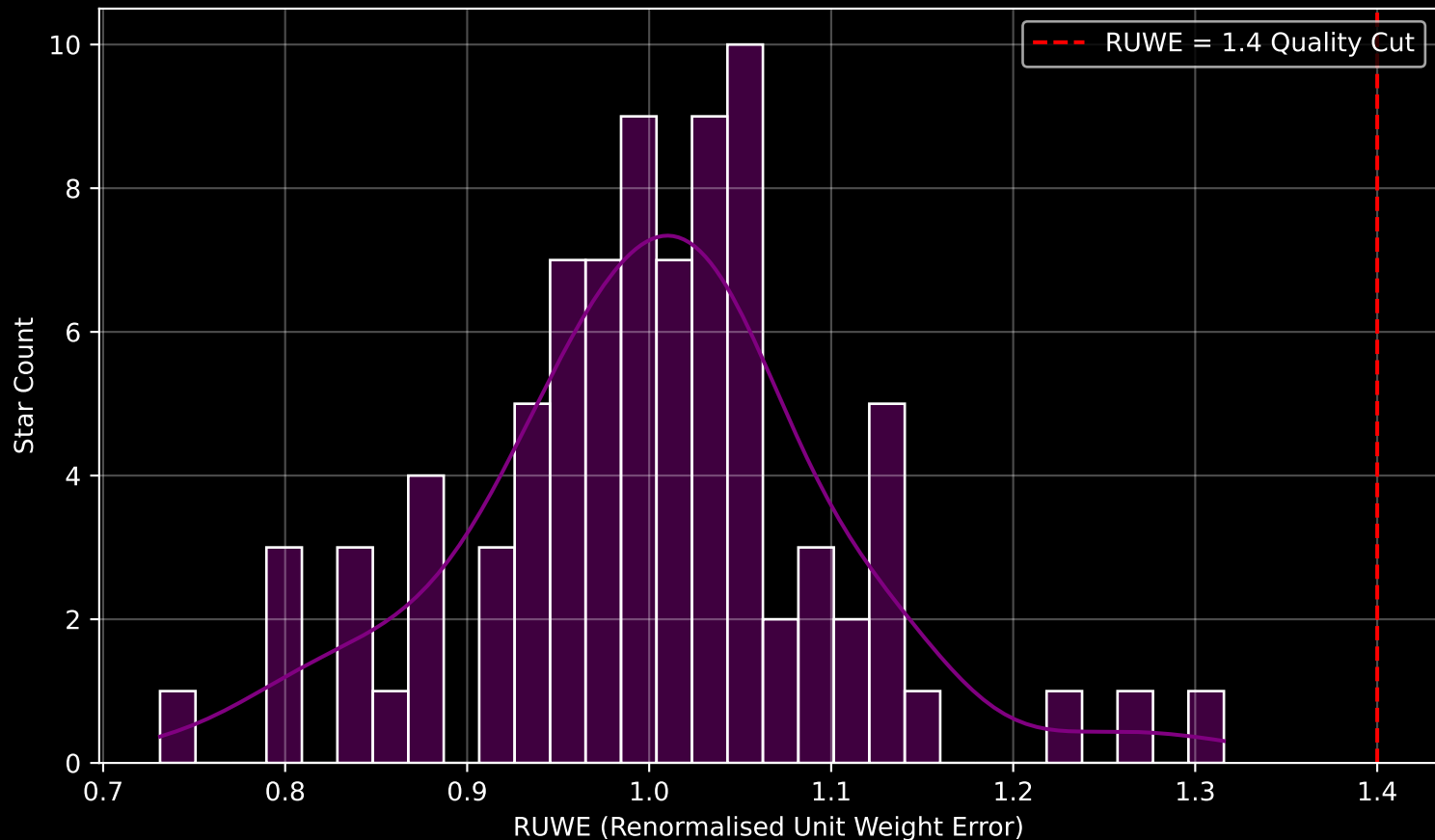
GAPOGEE DR17 Field [030+00_btx] RUWE Distribution (n= 85)
