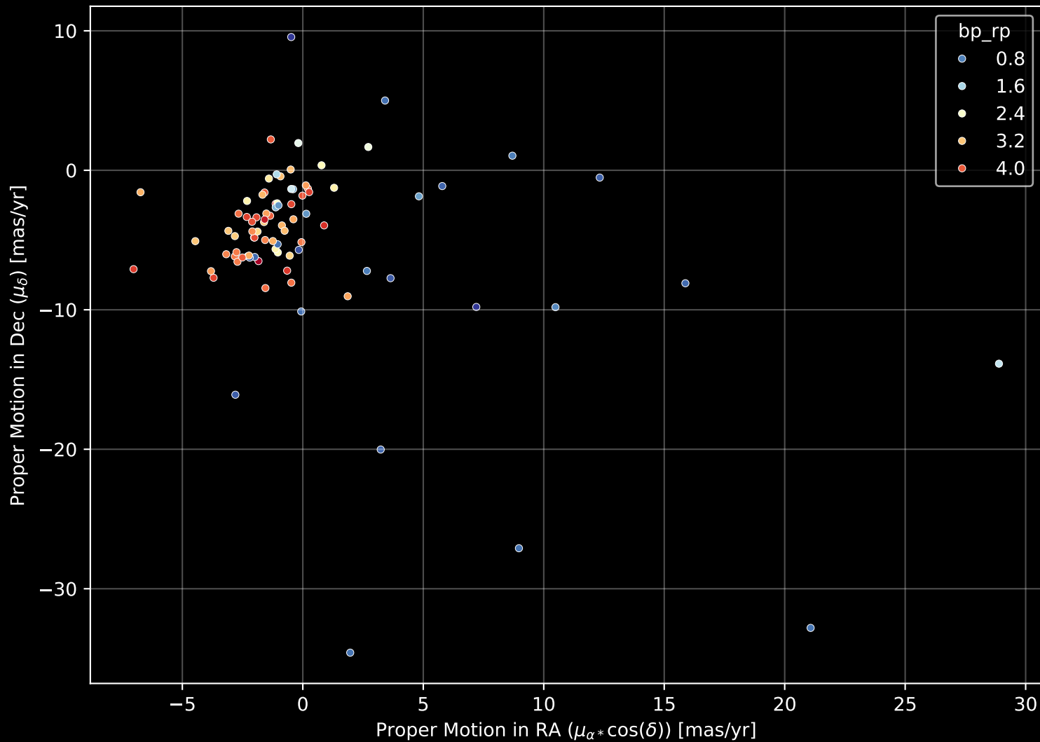
APOGEE DR17 Field: [030+00_btx] Proper Motion Diagram (n= 87)
