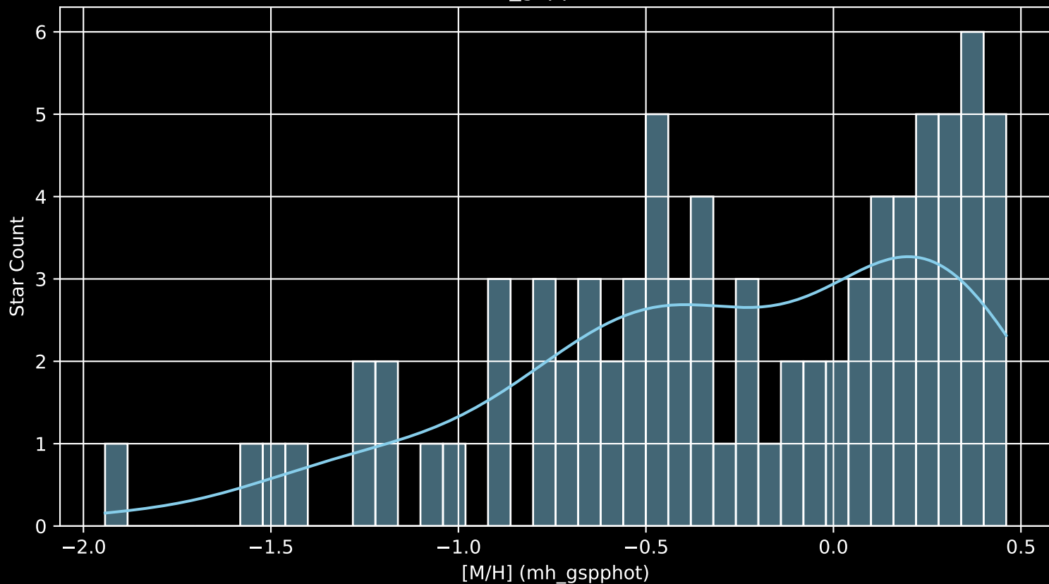
APOGEE DR17 Field: [030+00_btx [M/H] (mh_gspphot) (n= 81)
