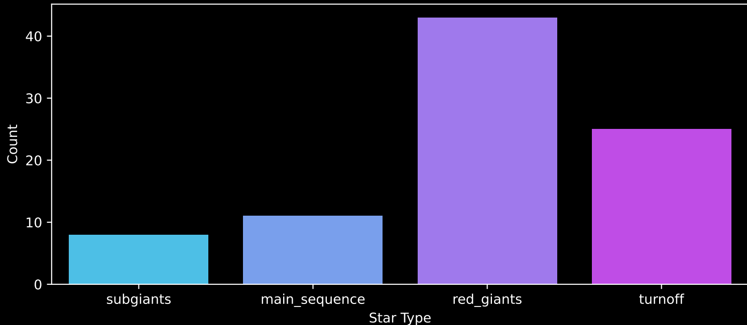
APOGEE DR17 Field: [030+00_btx] Count plot of Star Type
